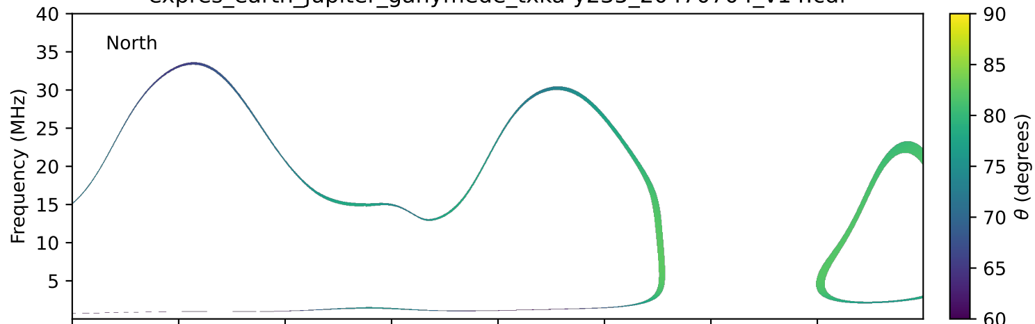
expres_earth_jupiter_ganymede_txka-y235_20470704_v14.cdf
