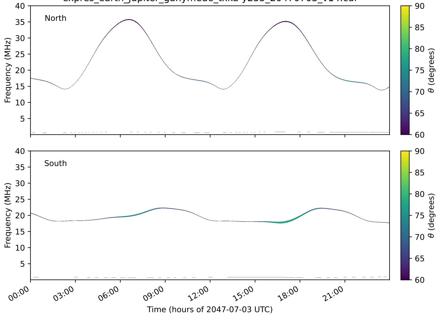
expres_earth_jupiter_ganymede_txka-y235_20470703_v14.cdf
