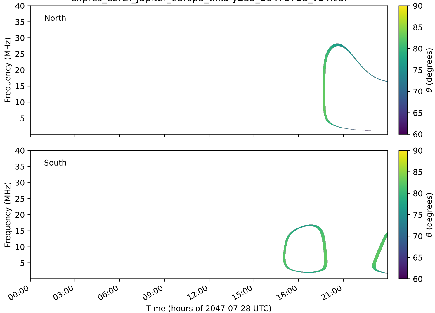
expres_earth_jupiter_europa_txka-y235_20470728_v14.cdf
