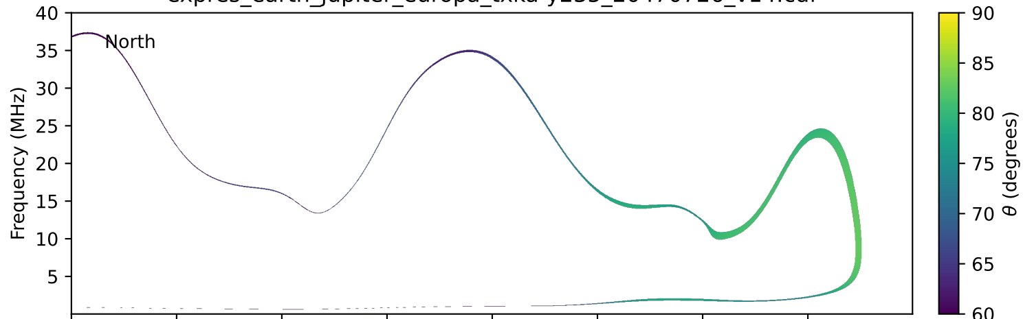
expres_earth_jupiter_europa_txka-y235_20470726_v14.cdf
