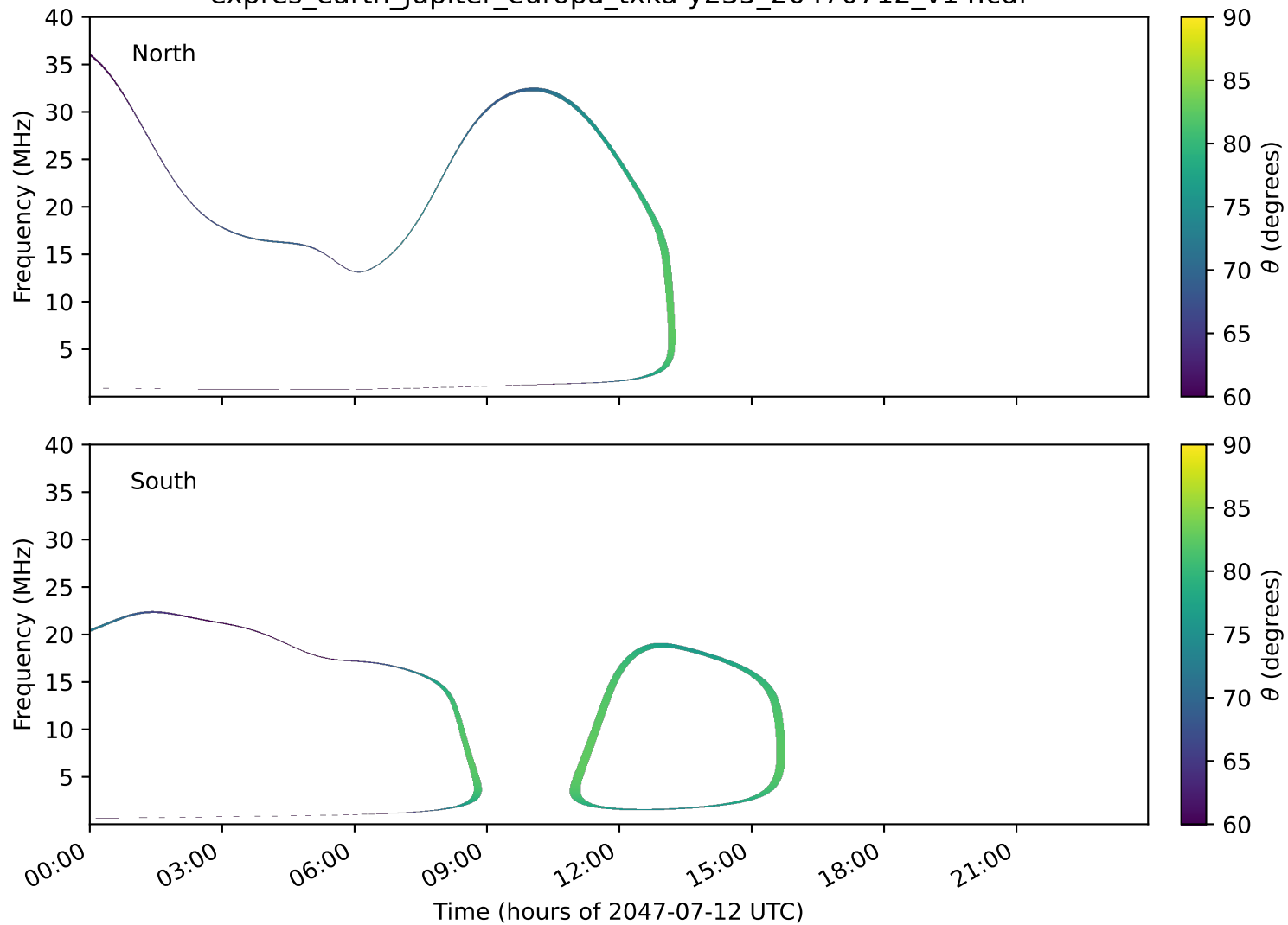
expres_earth_jupiter_europa_txka-y235_20470712_v14.cdf
