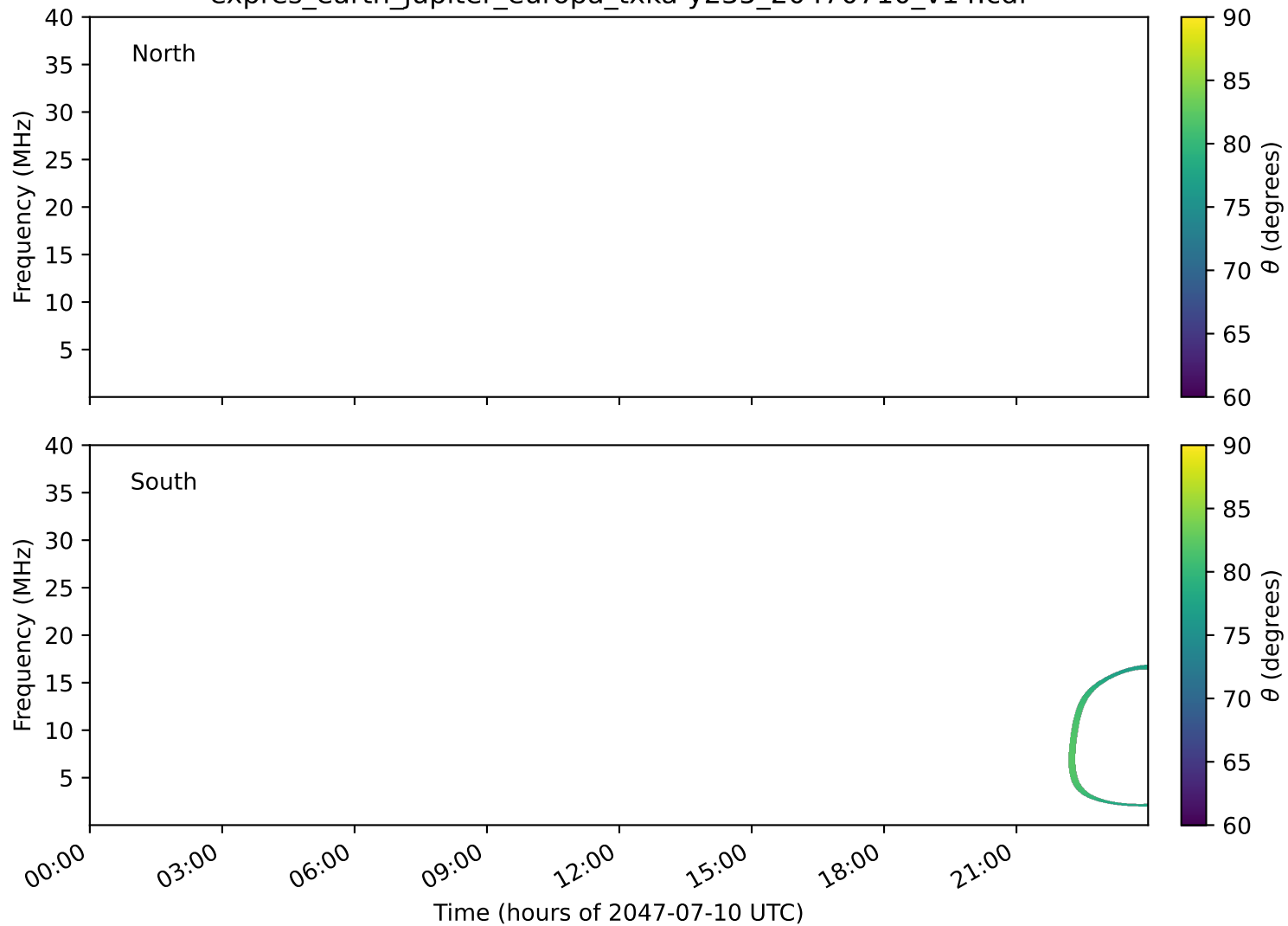
expres_earth_jupiter_europa_txka-y235_20470710_v14.cdf
