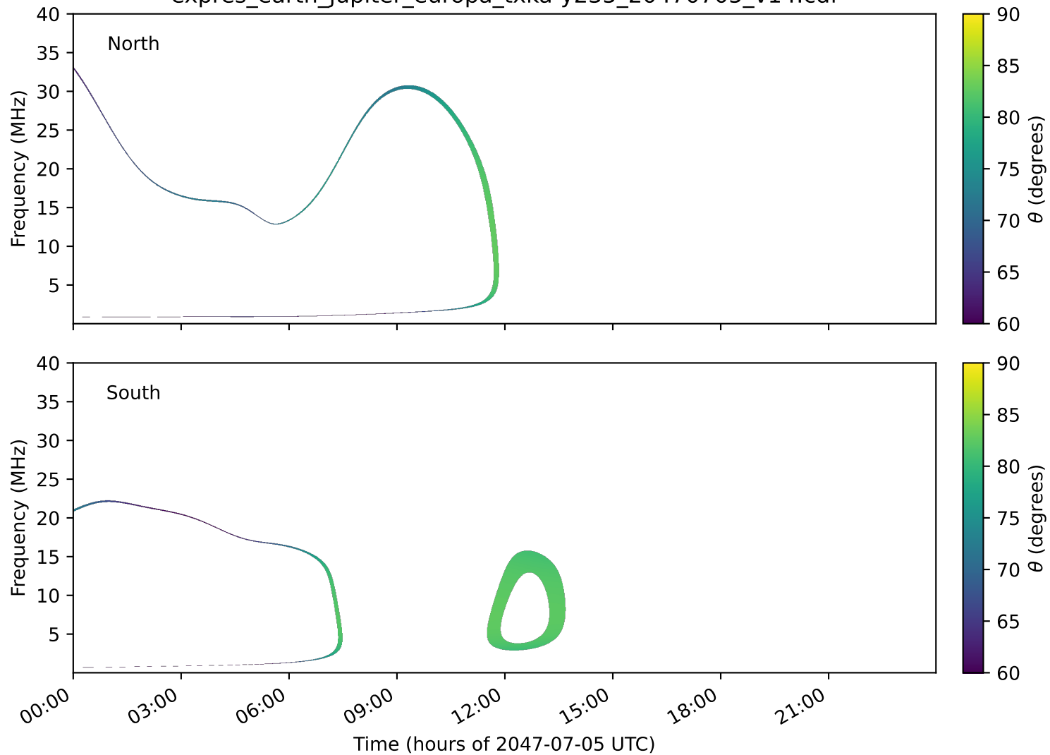
expres_earth_jupiter_europa_txka-y235_20470705_v14.cdf
