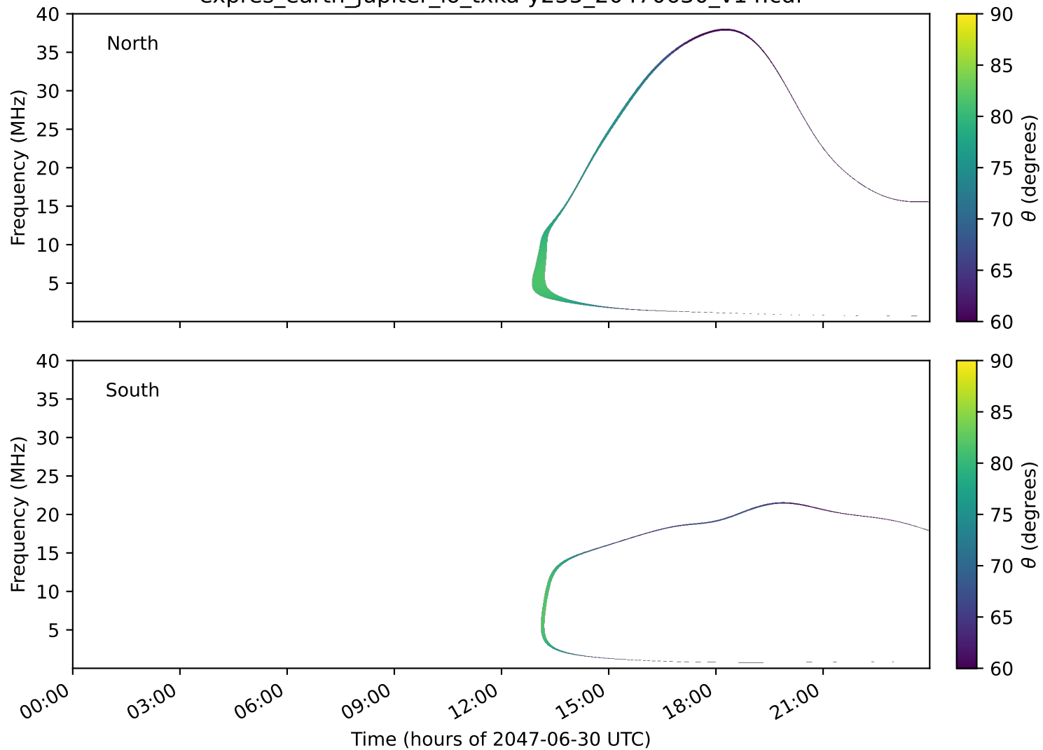
expres_earth_jupiter_io_txka-y235_20470630_v14.cdf
