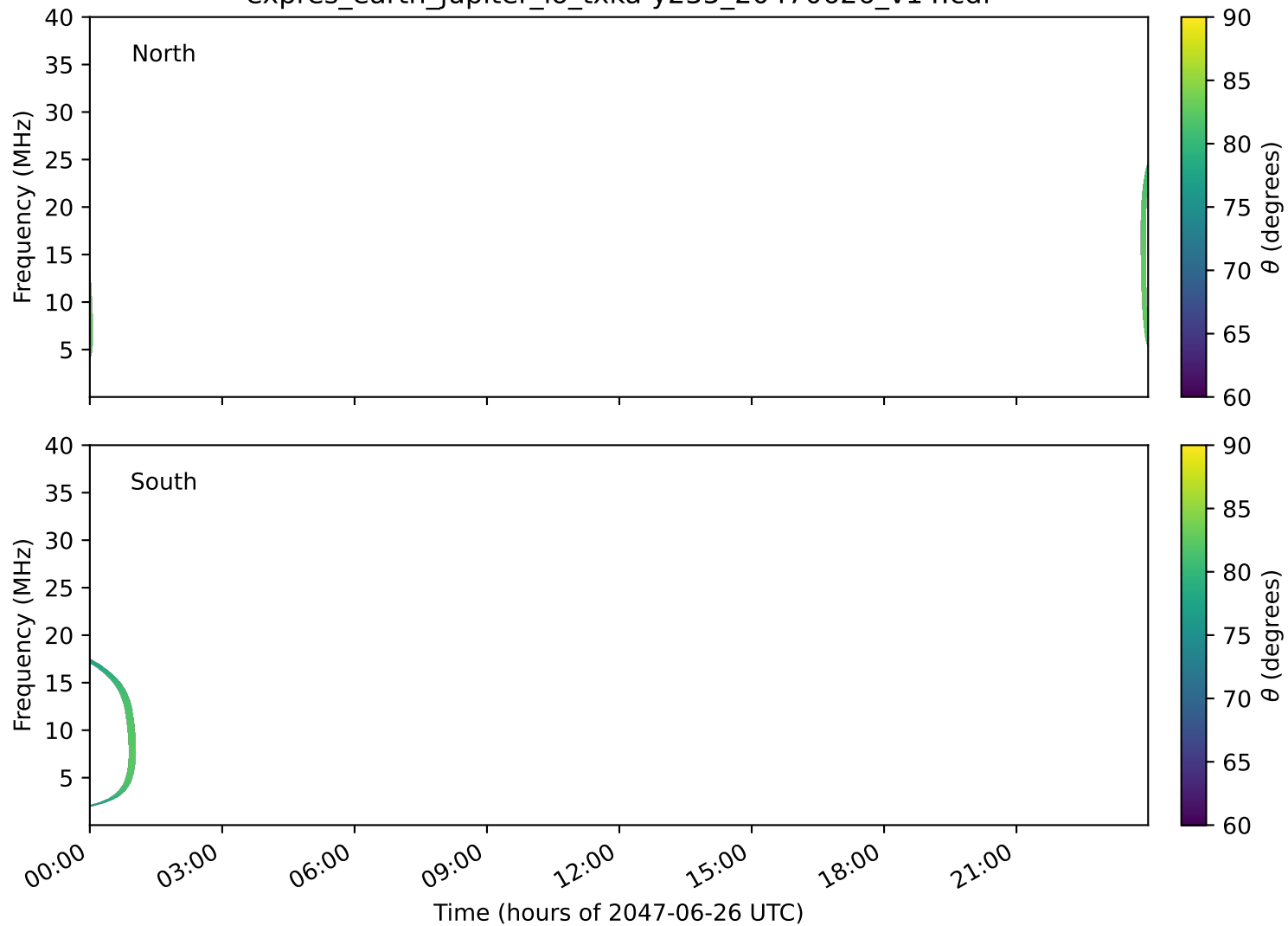
expres_earth_jupiter_io_txka-y235_20470626_v14.cdf
