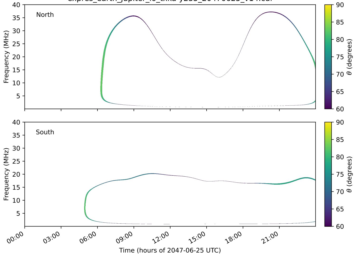
expres_earth_jupiter_io_txka-y235_20470625_v14.cdf
