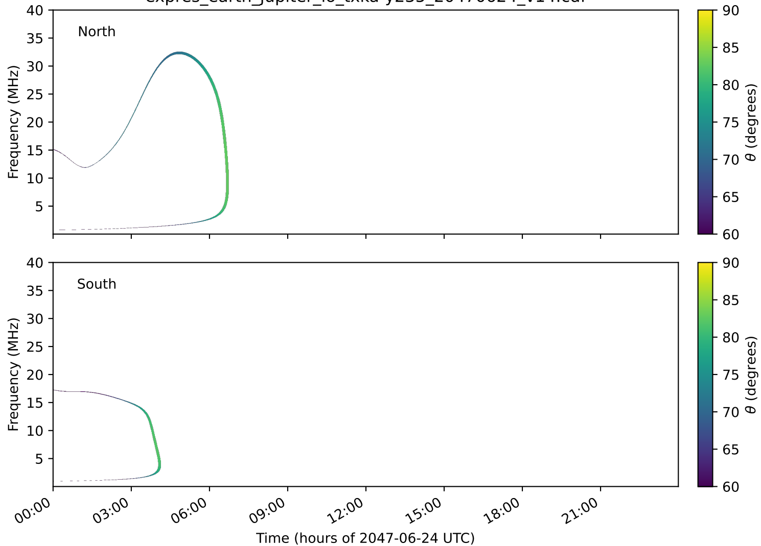
expres_earth_jupiter_io_txka-y235_20470624_v14.cdf
