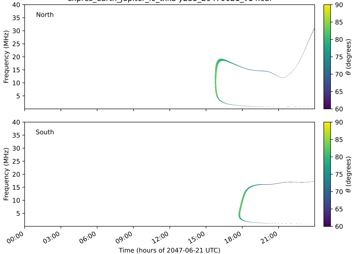
expres_earth_jupiter_io_txka-y235_20470621_v14.cdf
