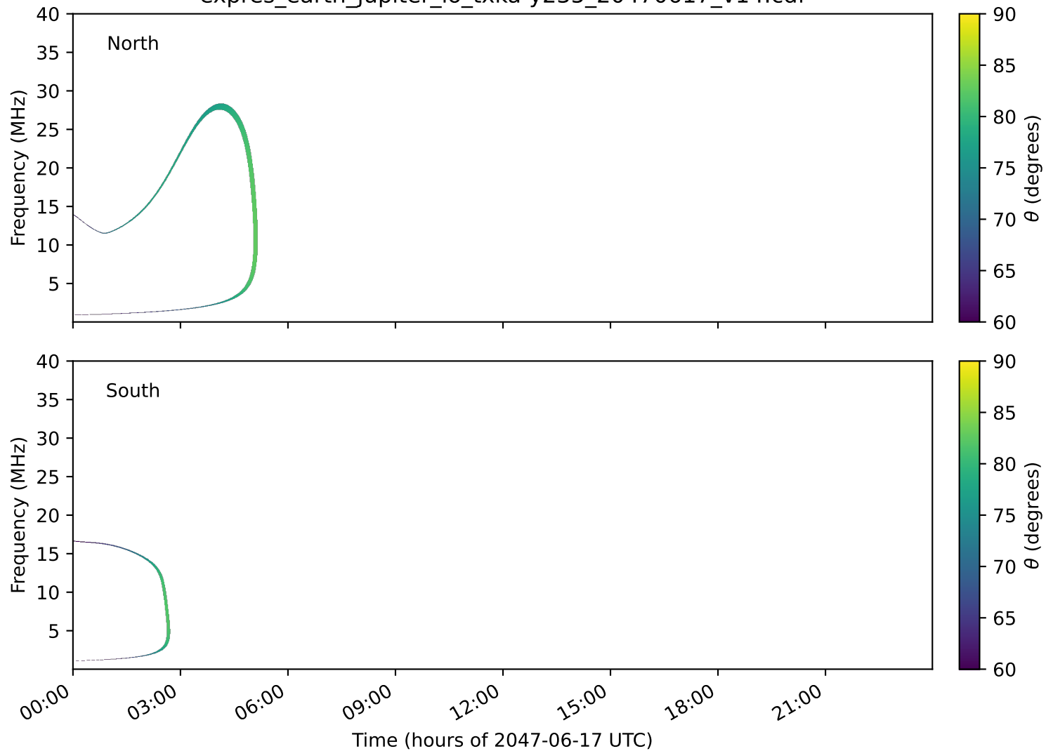
expres_earth_jupiter_io_txka-y235_20470617_v14.cdf
