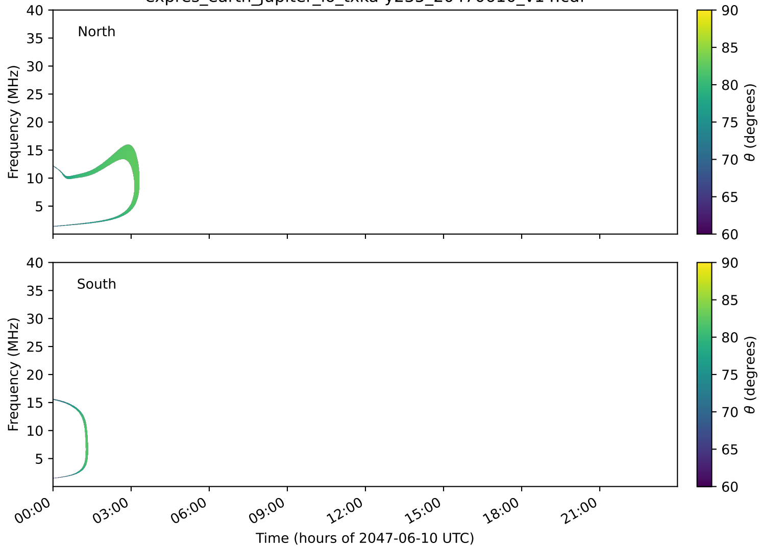
expres_earth_jupiter_io_txka-y235_20470610_v14.cdf
