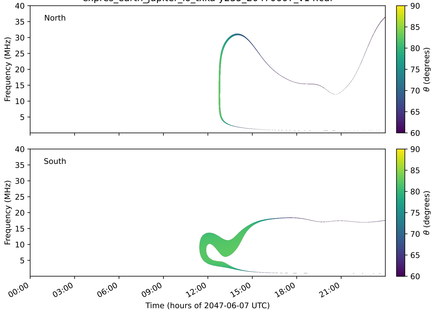
expres_earth_jupiter_io_txka-y235_20470607_v14.cdf
