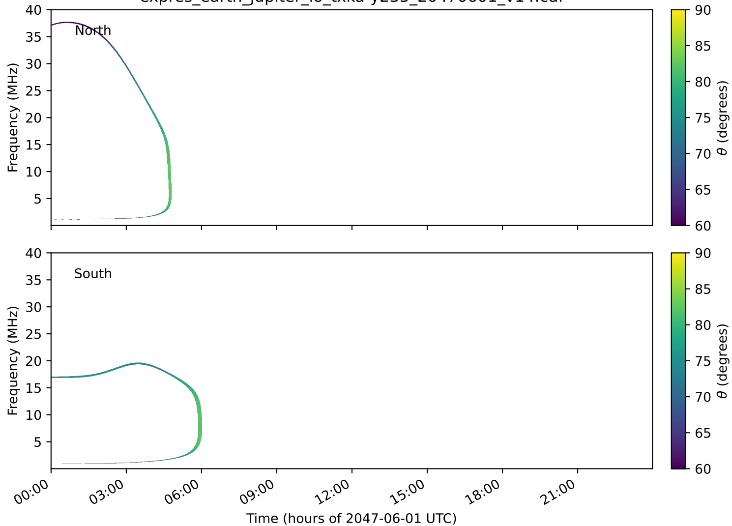
expres_earth_jupiter_io_txka-y235_20470601_v14.cdf
