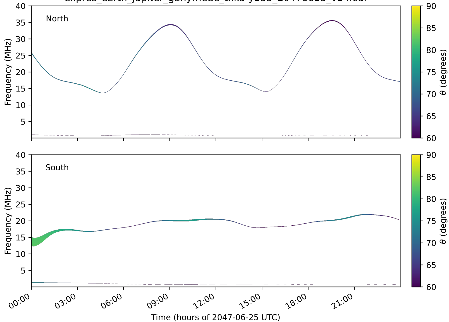
expres_earth_jupiter_ganymede_txka-y235_20470625_v14.cdf
