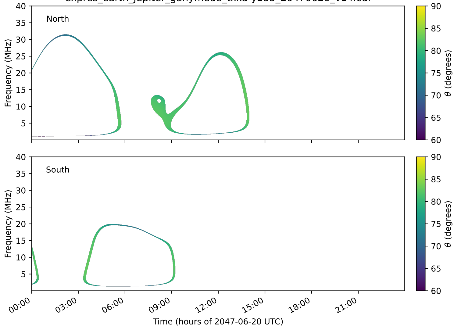
expres_earth_jupiter_ganymede_txka-y235_20470620_v14.cdf
