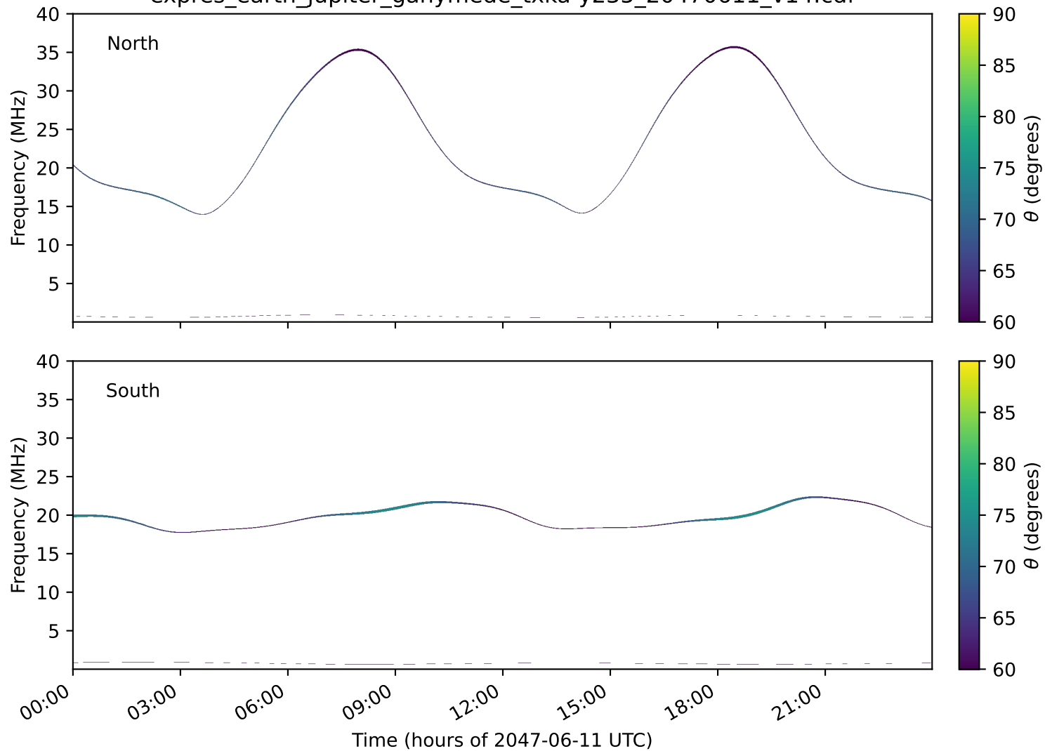
expres_earth_jupiter_ganymede_txka-y235_20470611_v14.cdf
