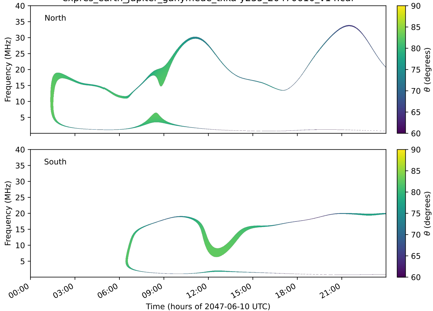
expres_earth_jupiter_ganymede_txka-y235_20470610_v14.cdf
