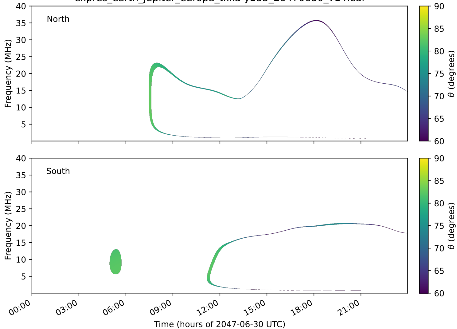
expres_earth_jupiter_europa_txka-y235_20470630_v14.cdf
