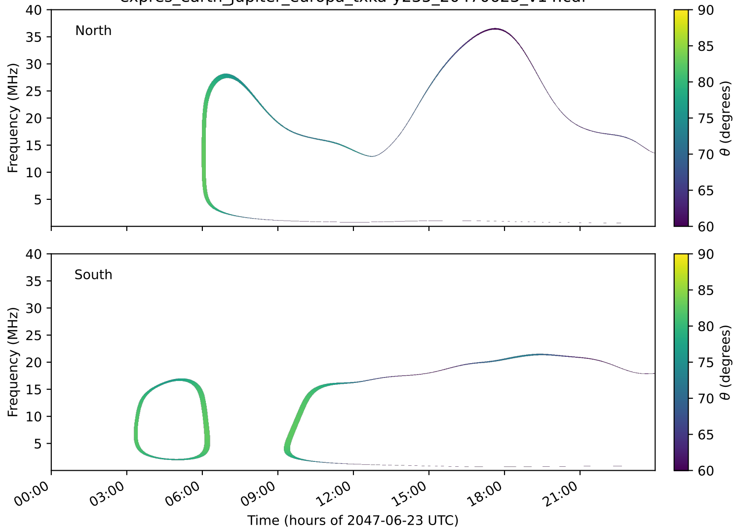
expres_earth_jupiter_europa_txka-y235_20470623_v14.cdf
