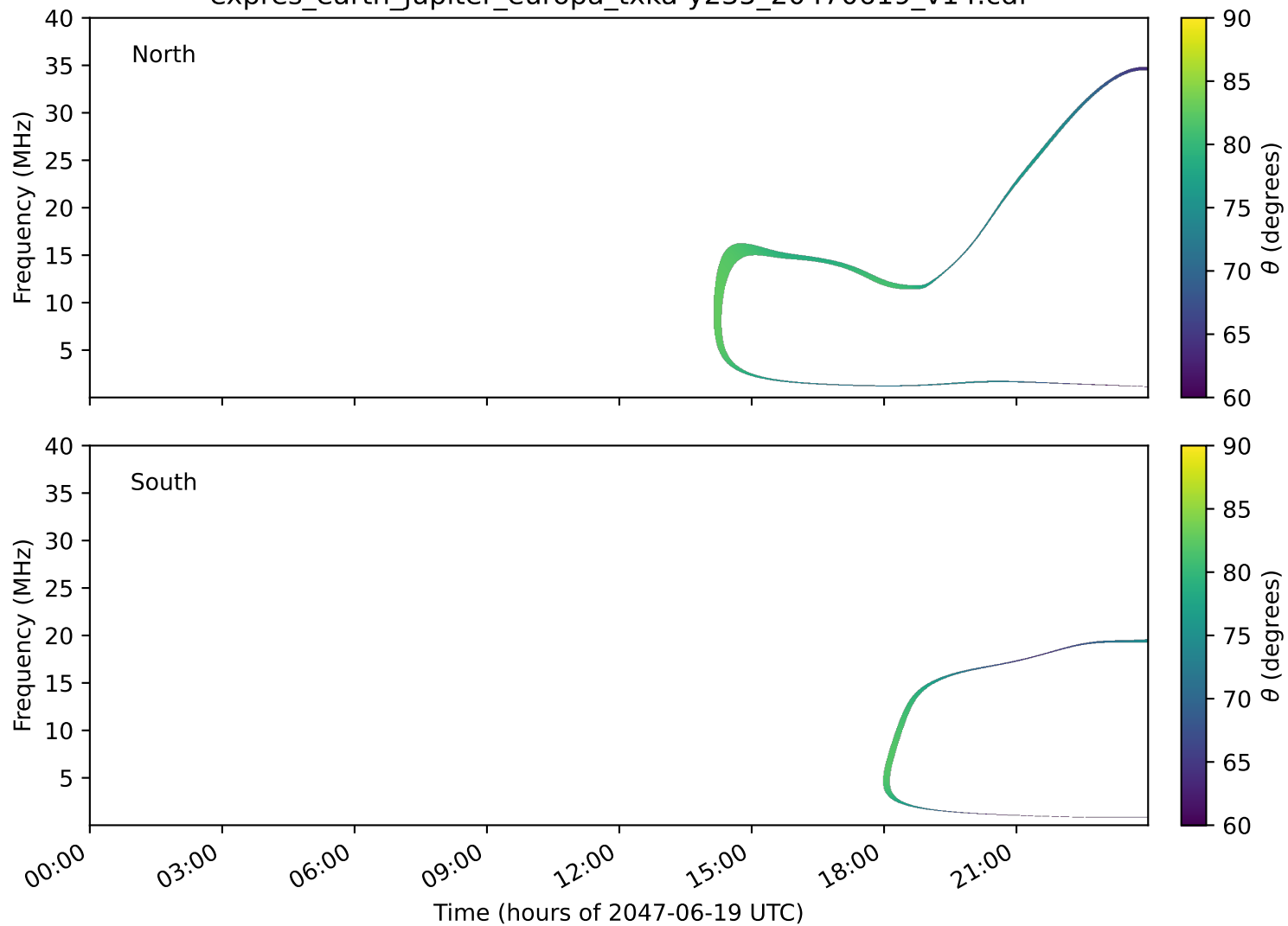
expres_earth_jupiter_europa_txka-y235_20470619_v14.cdf
