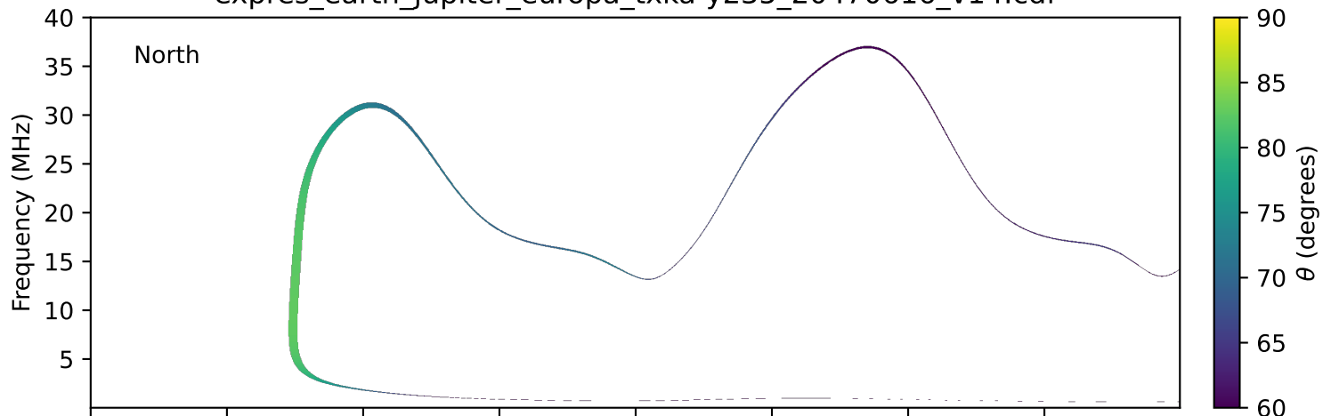
expres_earth_jupiter_europa_txka-y235_20470616_v14.cdf
