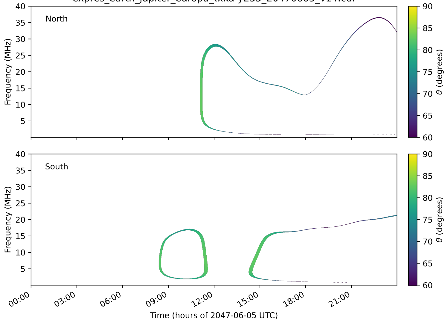
expres_earth_jupiter_europa_txka-y235_20470605_v14.cdf
