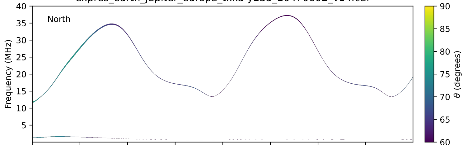
expres_earth_jupiter_europa_txka-y235_20470602_v14.cdf
