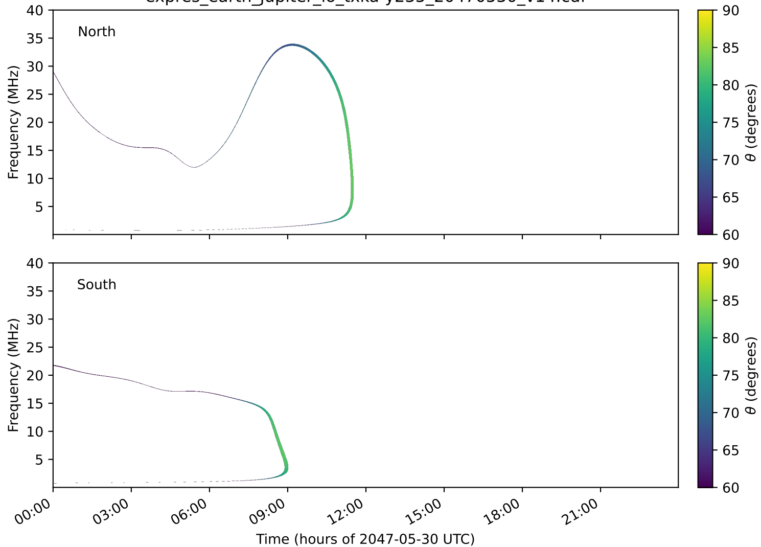
expres_earth_jupiter_io_txka-y235_20470530_v14.cdf
