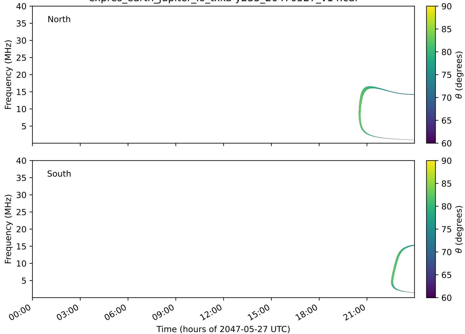
expres_earth_jupiter_io_txka-y235_20470527_v14.cdf
