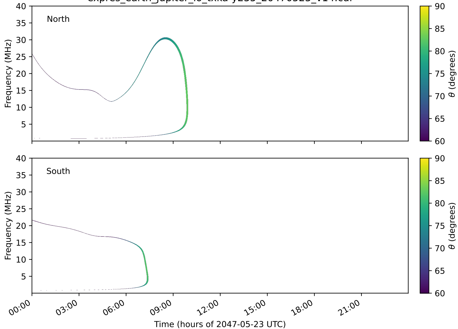
expres_earth_jupiter_io_txka-y235_20470523_v14.cdf
