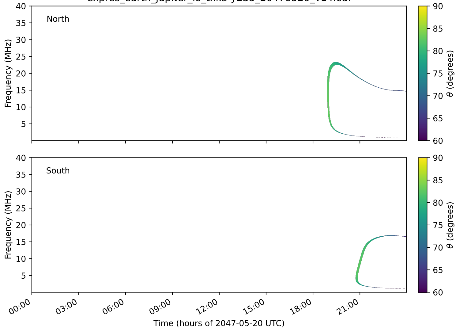
expres_earth_jupiter_io_txka-y235_20470520_v14.cdf
