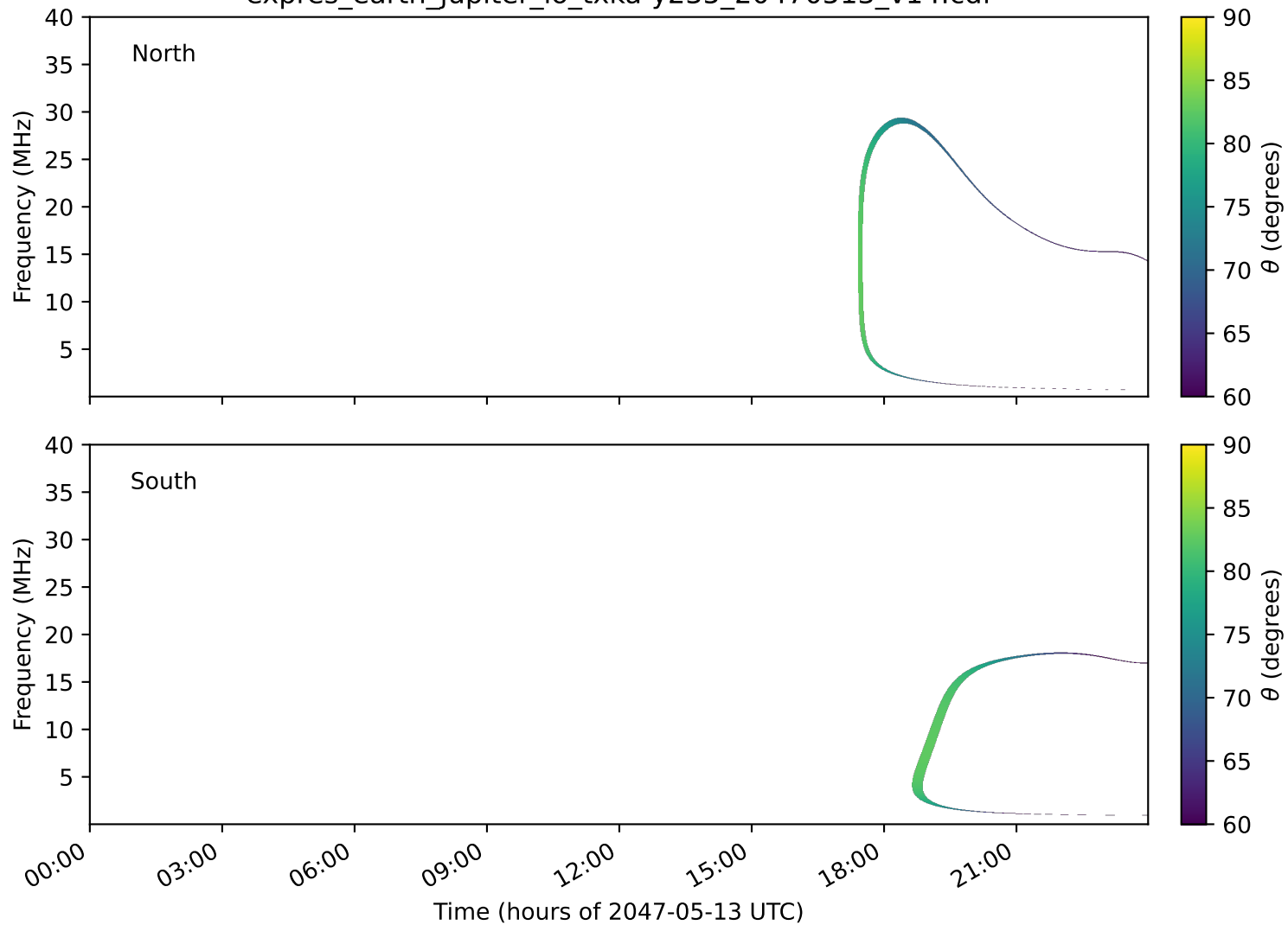
expres_earth_jupiter_io_txka-y235_20470513_v14.cdf
