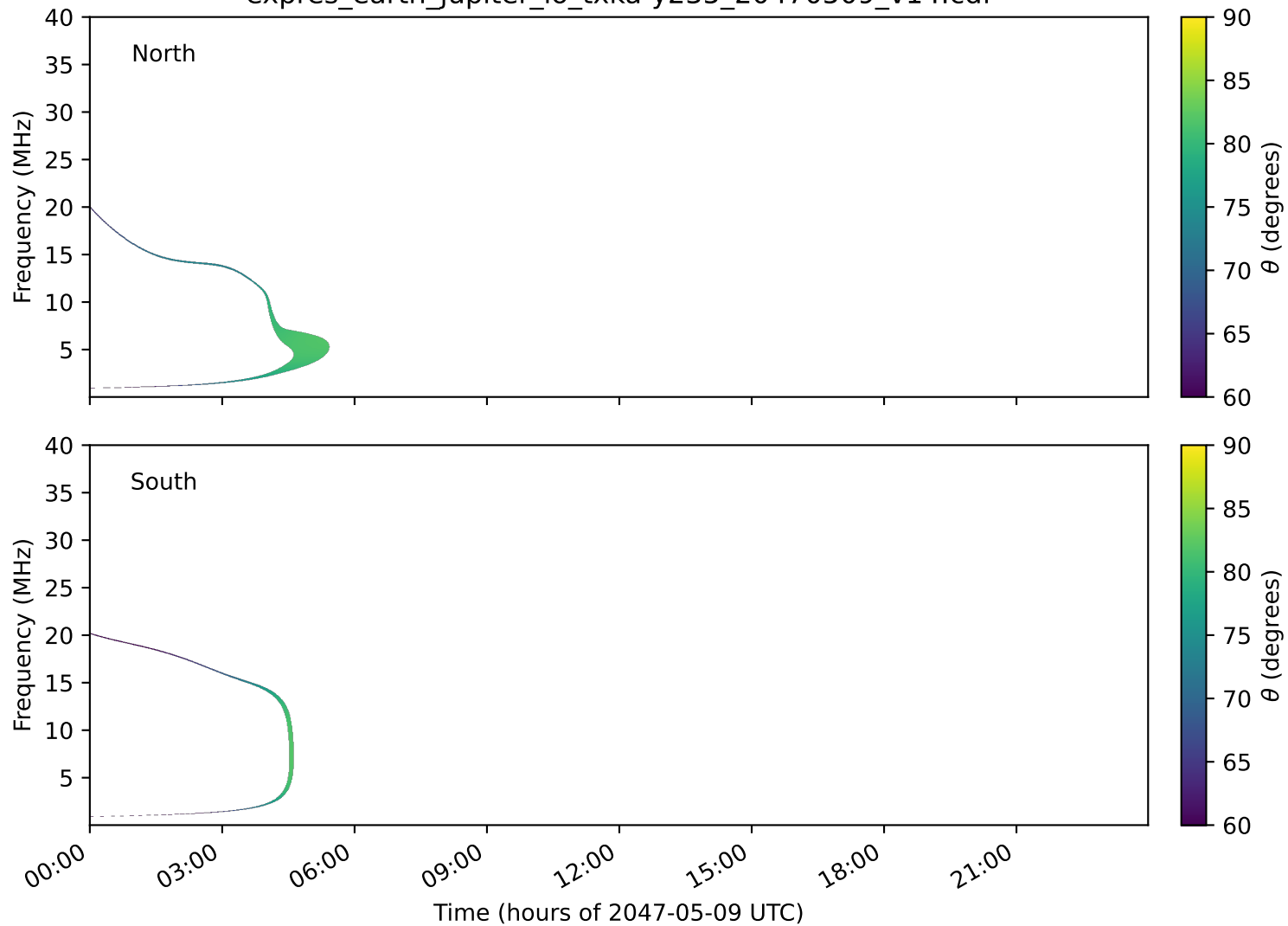
expres_earth_jupiter_io_txka-y235_20470509_v14.cdf
