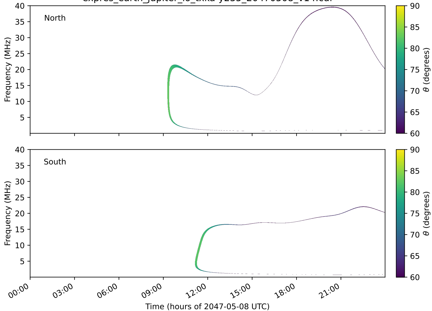
expres_earth_jupiter_io_txka-y235_20470508_v14.cdf
