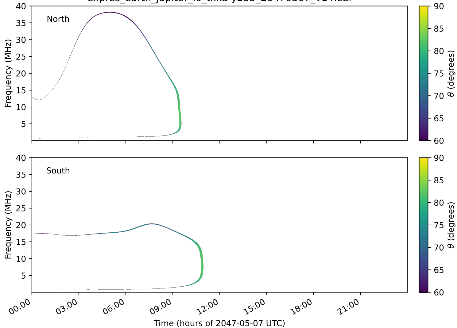
expres_earth_jupiter_io_txka-y235_20470507_v14.cdf
