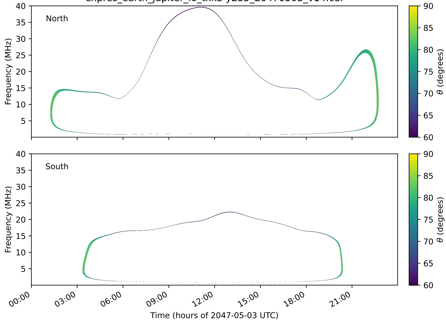
expres_earth_jupiter_io_txka-y235_20470503_v14.cdf
