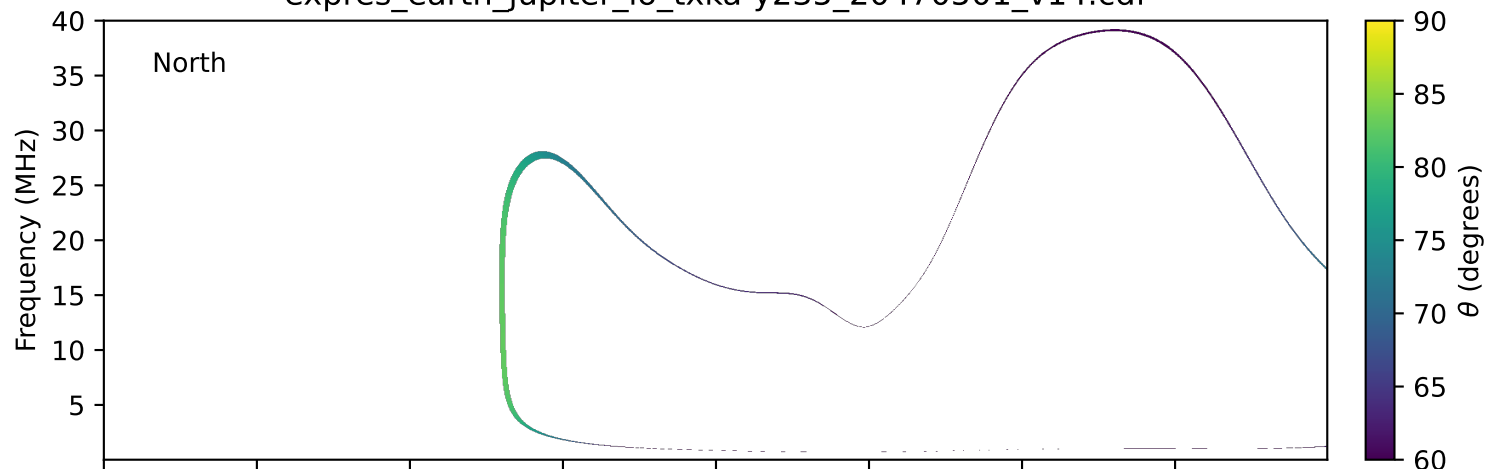
expres_earth_jupiter_io_txka-y235_20470501_v14.cdf
