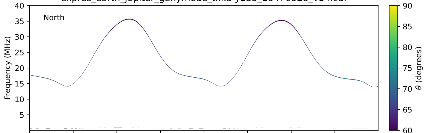
expres_earth_jupiter_ganymede_txka-y235_20470528_v14.cdf
