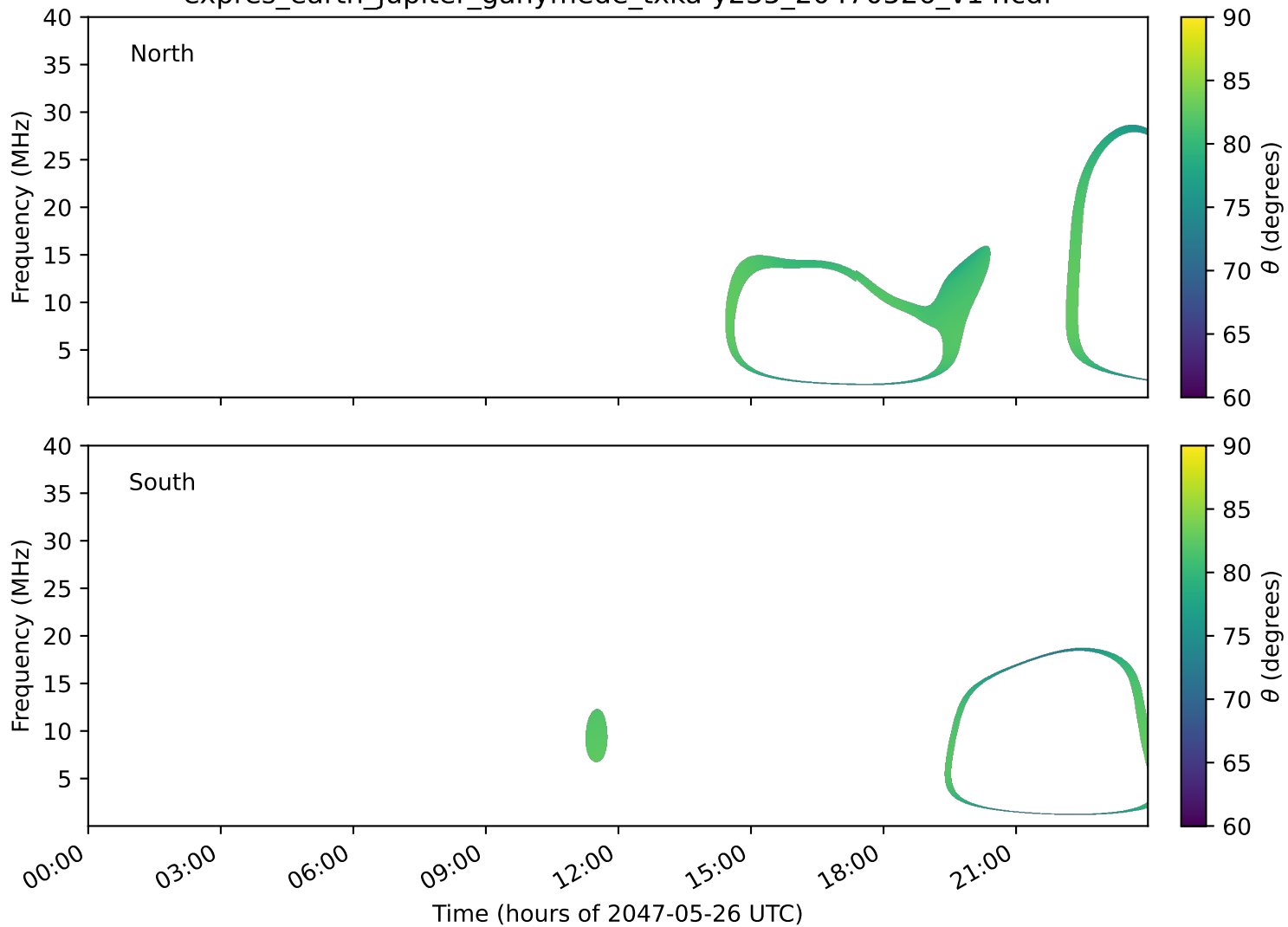
expres_earth_jupiter_ganymede_txka-y235_20470526_v14.cdf
