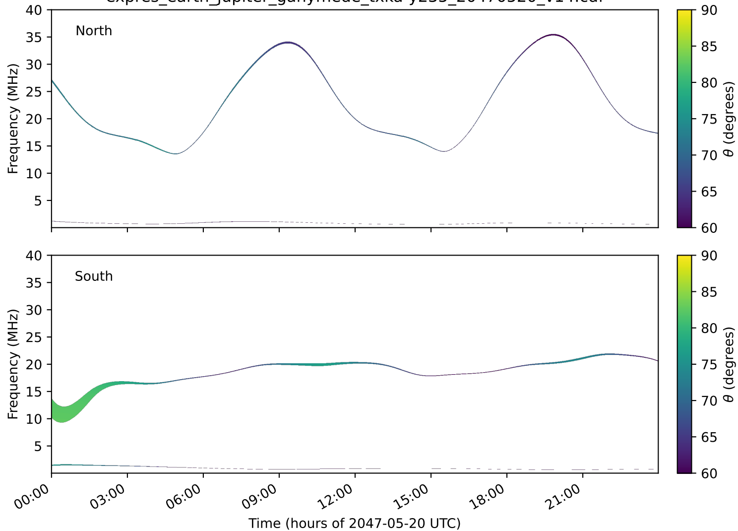
expres_earth_jupiter_ganymede_txka-y235_20470520_v14.cdf
