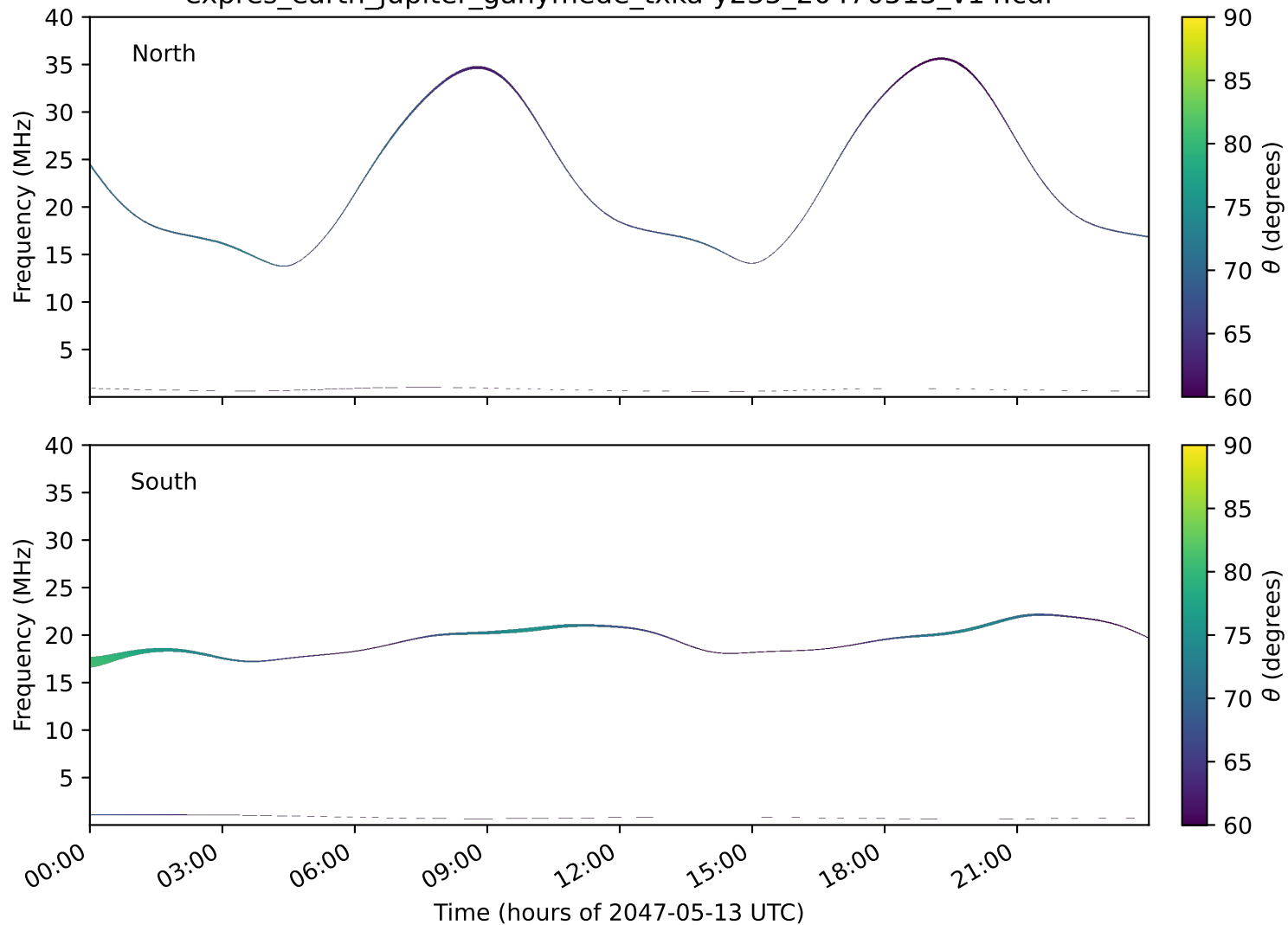
expres_earth_jupiter_ganymede_txka-y235_20470513_v14.cdf
