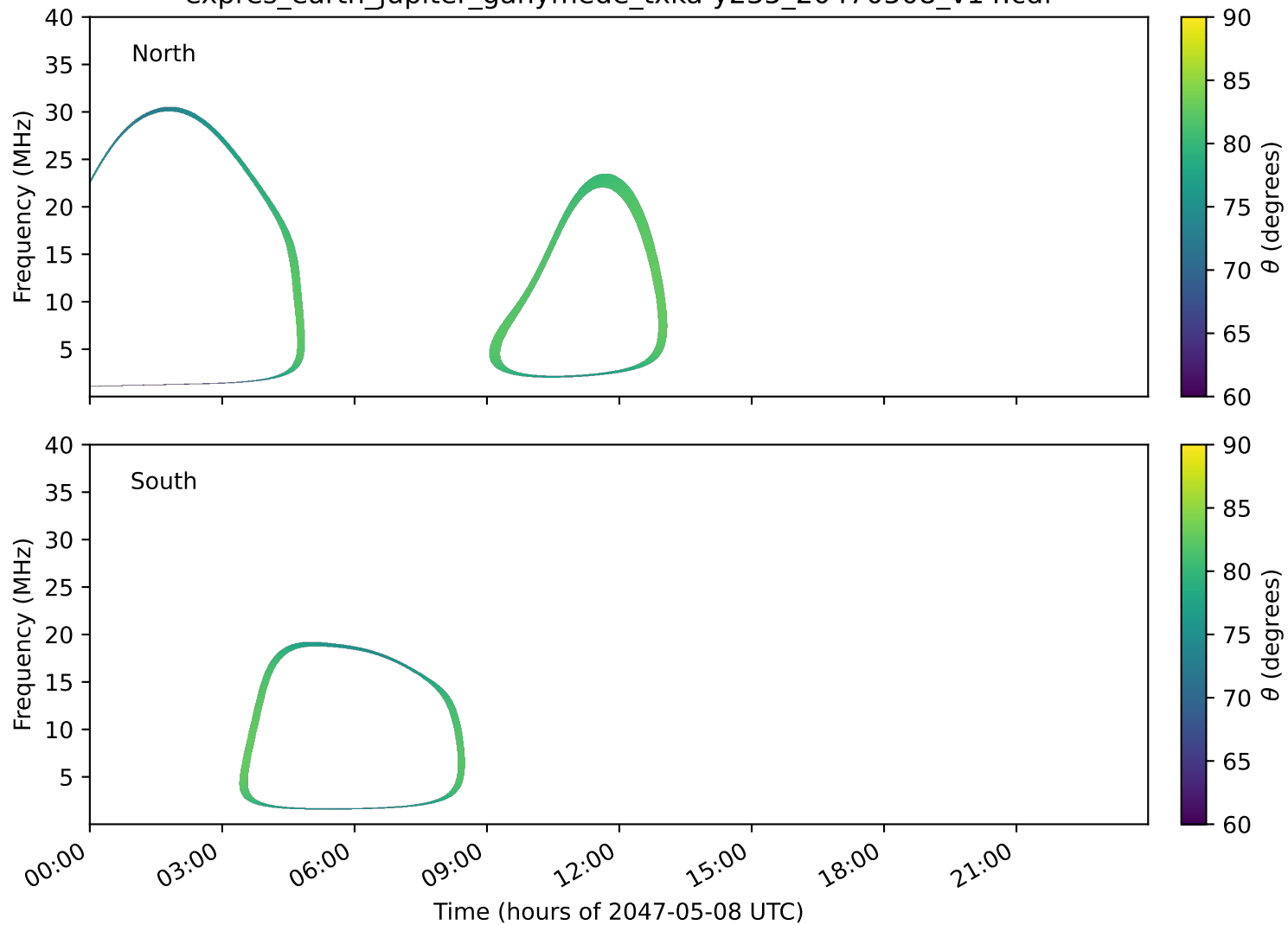
expres_earth_jupiter_ganymede_txka-y235_20470508_v14.cdf
