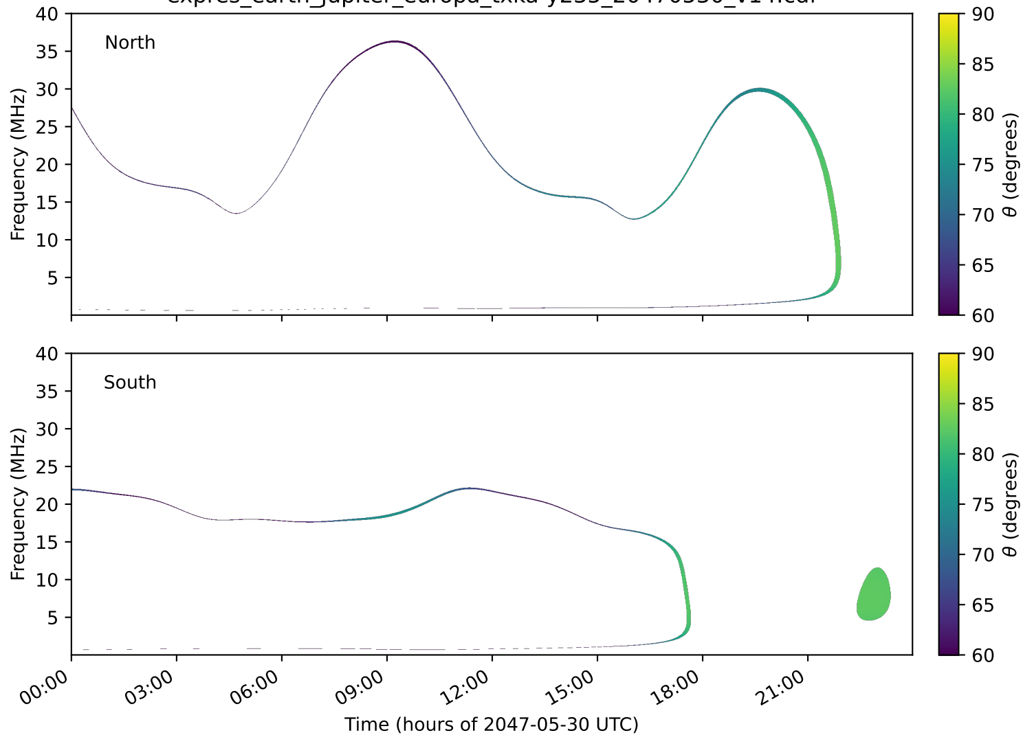
expres_earth_jupiter_europa_txka-y235_20470530_v14.cdf
