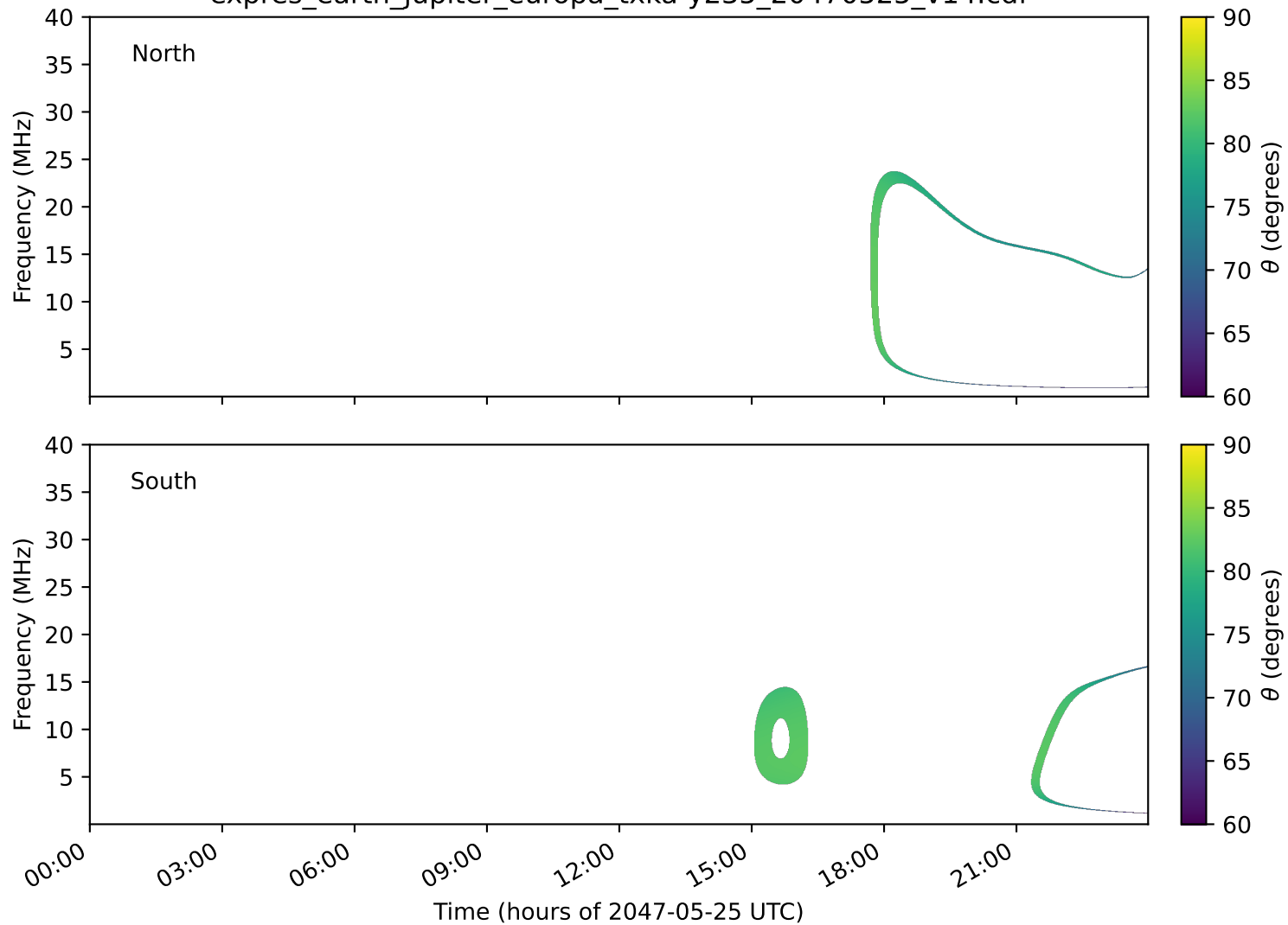
expres_earth_jupiter_europa_txka-y235_20470525_v14.cdf
