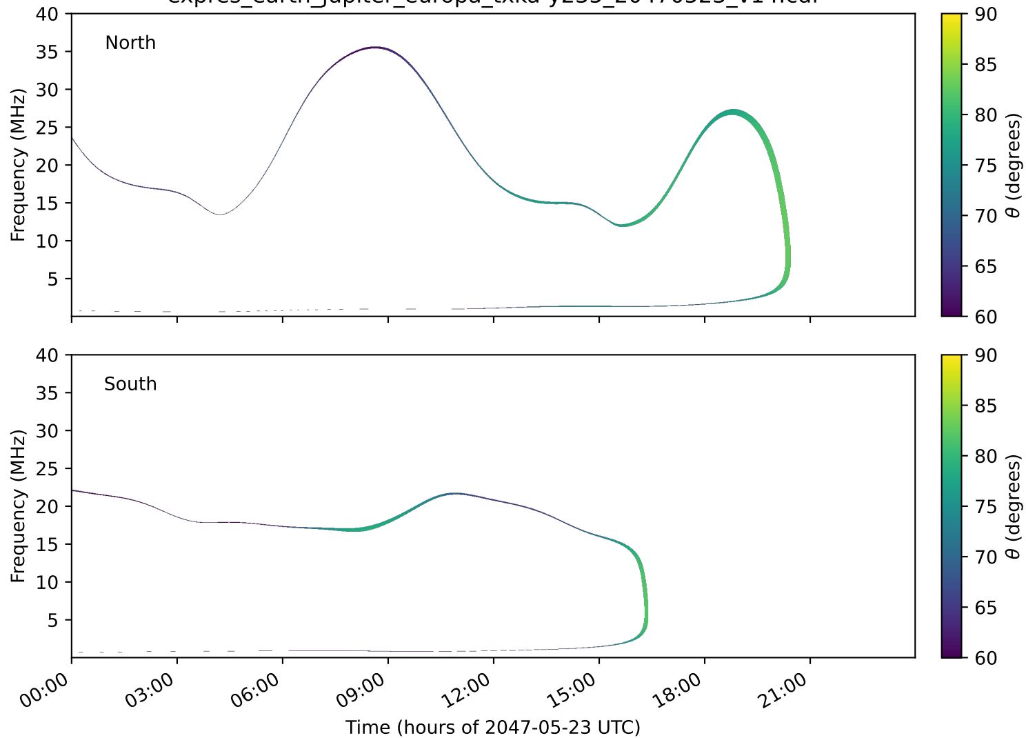
expres_earth_jupiter_europa_txka-y235_20470523_v14.cdf
