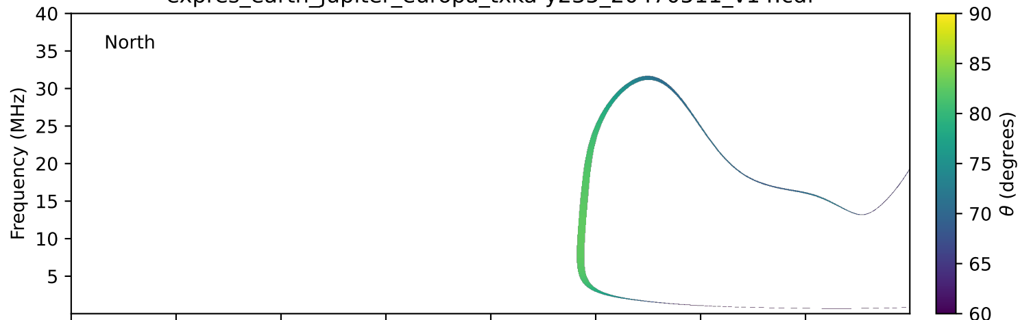
expres_earth_jupiter_europa_txka-y235_20470511_v14.cdf
