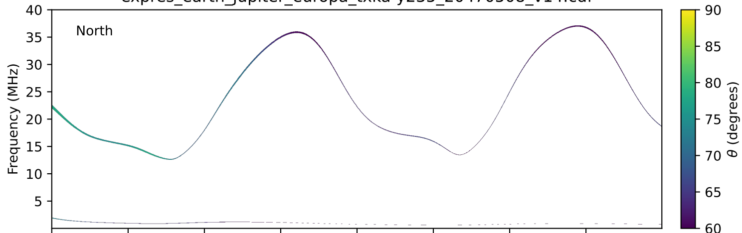
expres_earth_jupiter_europa_txka-y235_20470508_v14.cdf
