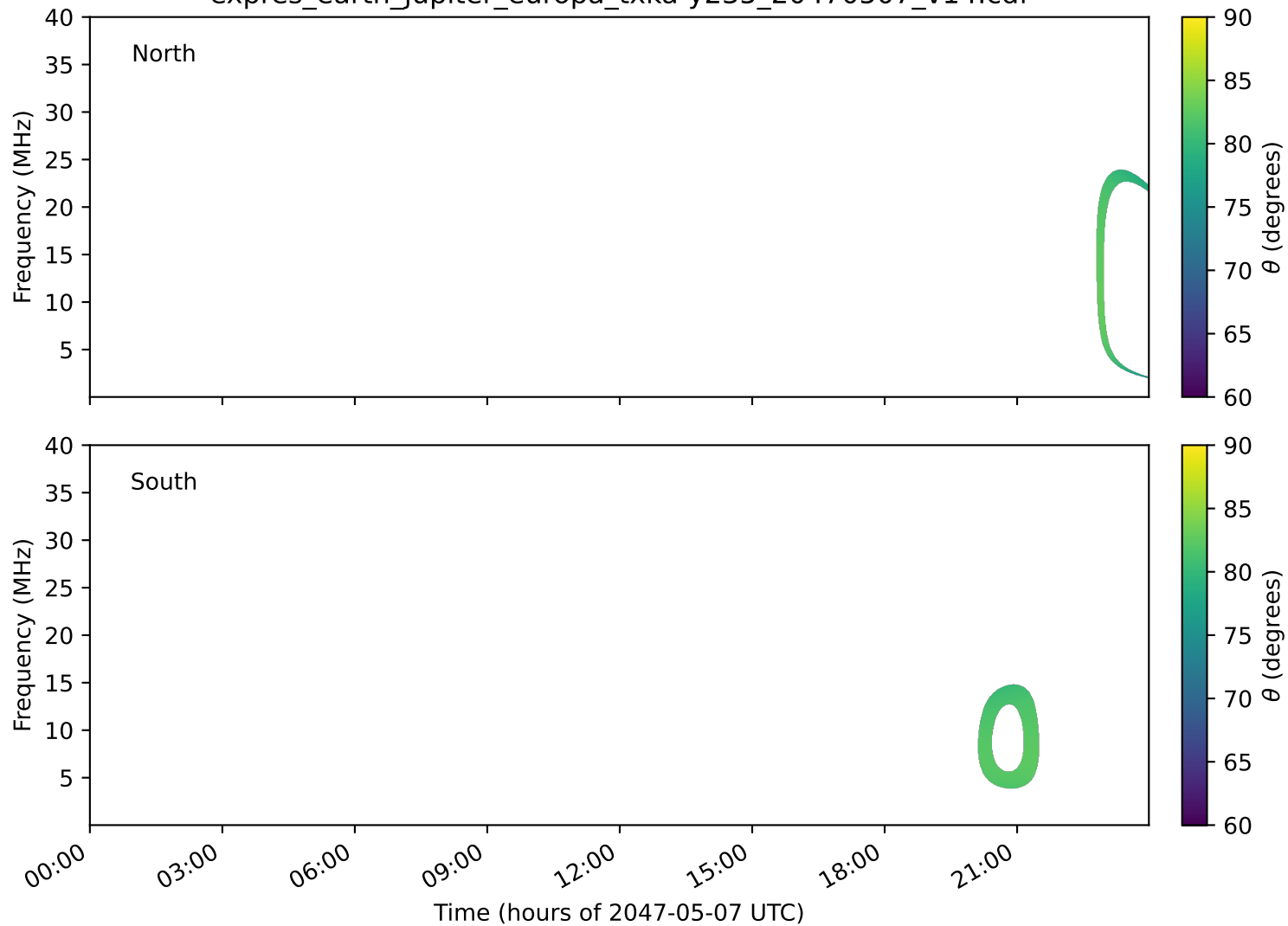
expres_earth_jupiter_europa_txka-y235_20470507_v14.cdf
