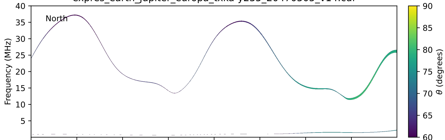
expres_earth_jupiter_europa_txka-y235_20470505_v14.cdf
