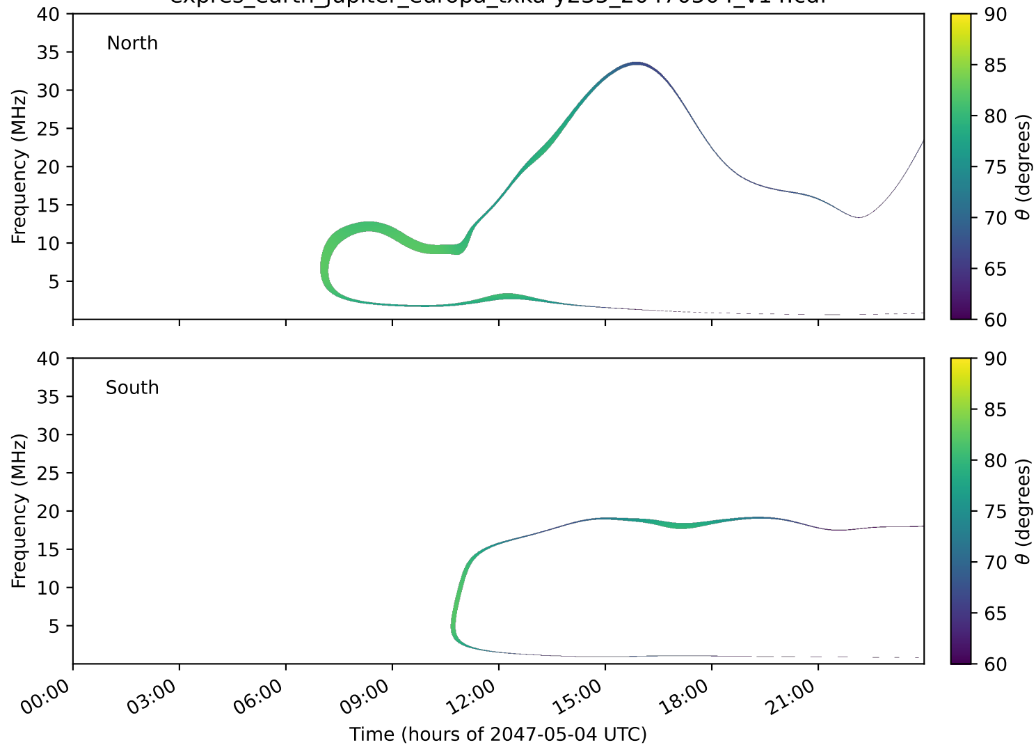
expres_earth_jupiter_europa_txka-y235_20470504_v14.cdf
