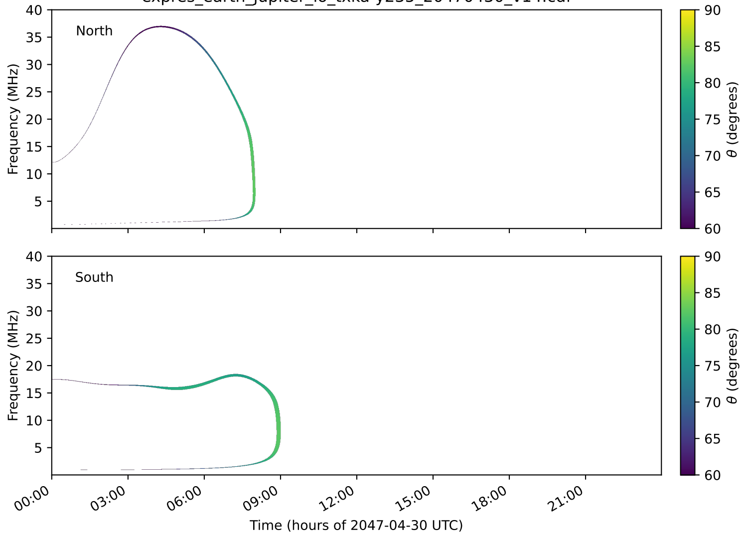
expres_earth_jupiter_io_txka-y235_20470430_v14.cdf
